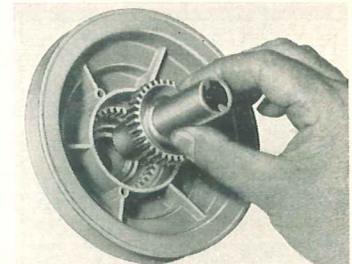
How the floating sleeve is engaged with the internal gear in the pulley is shown in the first photo. This forms a clutch which permits the sleeve to float in all directions but one.
